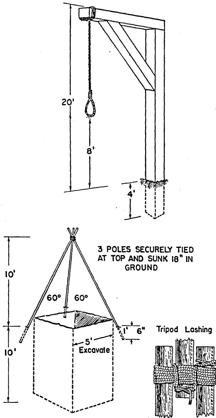
Figure 4. Emergency gallows, post type and tripod type.
