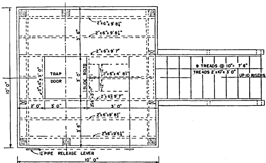
PLATFORM AND STAIR PLAN AT SECTION A-A SCALE 1/2" = 1'
