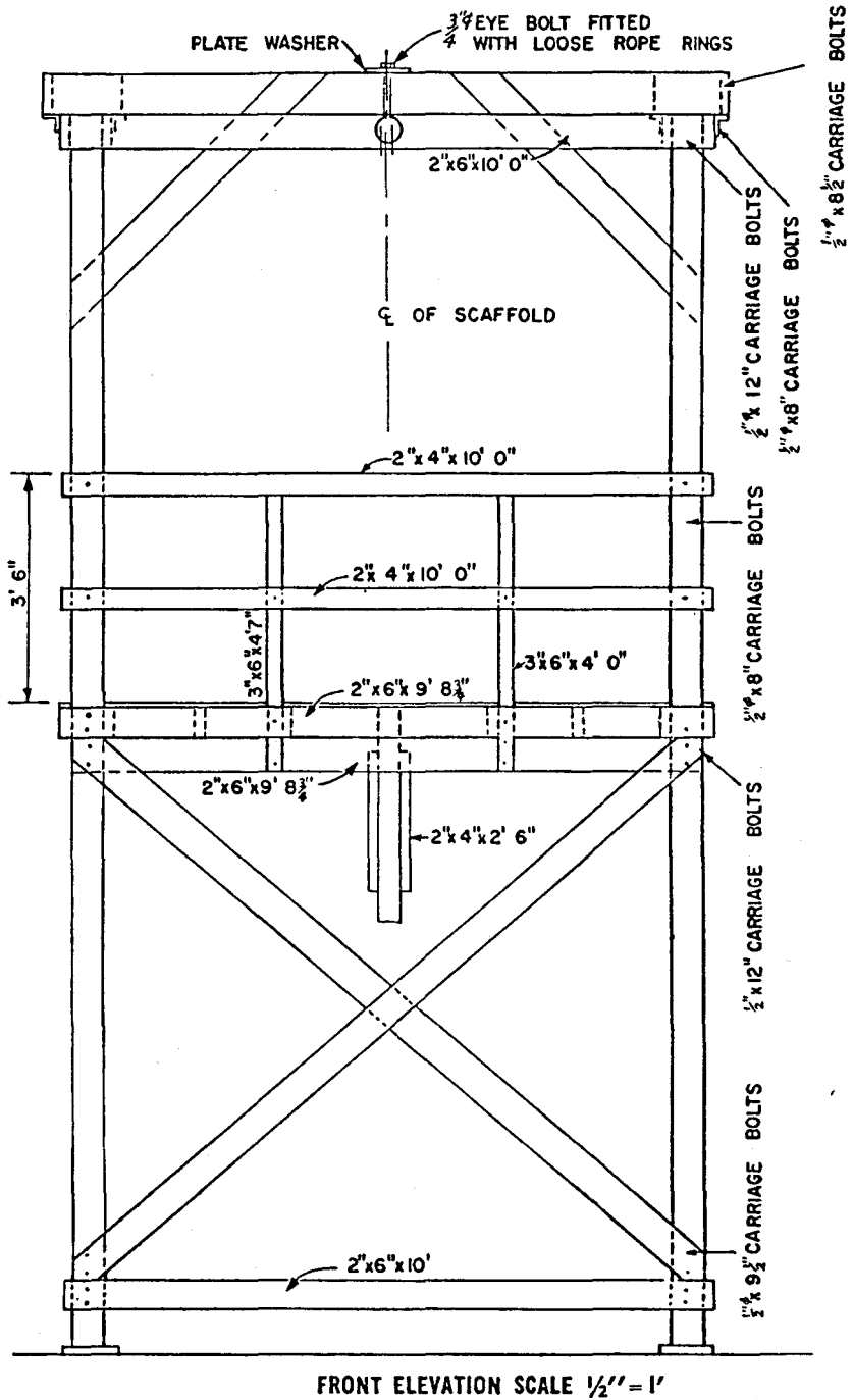
Figure 2 (2). Permanent scaffold, front elevation.
